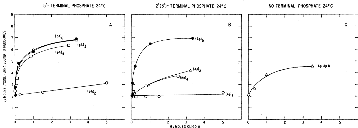
Fig. 9. A , B , and C , Relation between template activity and oligoA concentration, chain-length, and end group. The activity of oligoA with 5'-terminal phosphate is shown in Fig. 9 A ; preparation without terminal phosphate in Fig. 9 C . The symbols indicate the chain-length of oligoA as follows: ○ 2; △ 3; □ 4; ● 6. Each 50 \mu l reaction mixture contained the components specified under methods; 15.9 \mu μmole of C^{14} -Lys-sRNA (1780 count/min, 0.562 A^{260} units); and the oligoA preparation specified. Incubation was at 24°C for 20 minutes. Oligonucleotide preparations (pA) 6 , No. 599 and (Ap) 4 , No. 591, containing the contaminants specified under Methods , were used in this experiment.
